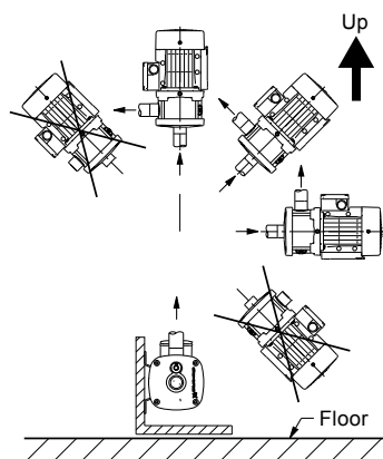
Fig. 11 Positions of CM and CME pumps
