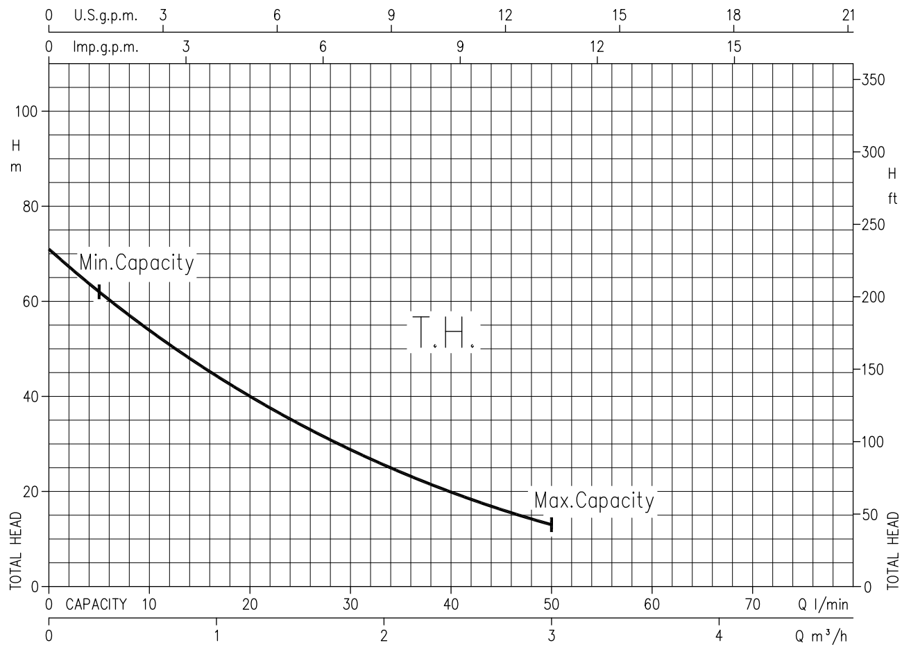
PRA 1.00 - Impeller diameter = 70.8 mm
